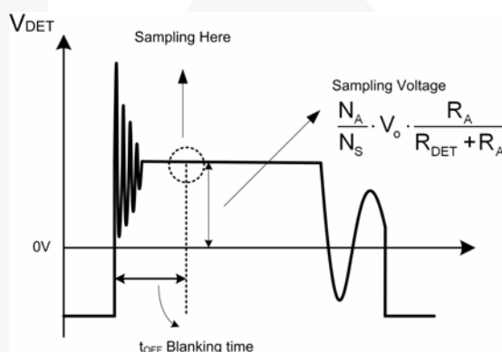
Figure 23. Voltage Sampled After 4μs Blanking Time After Switch-off Sequence
