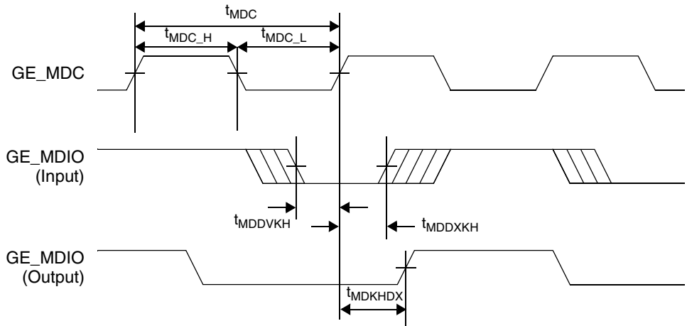
Figure 24. MII Management Interface Timing
