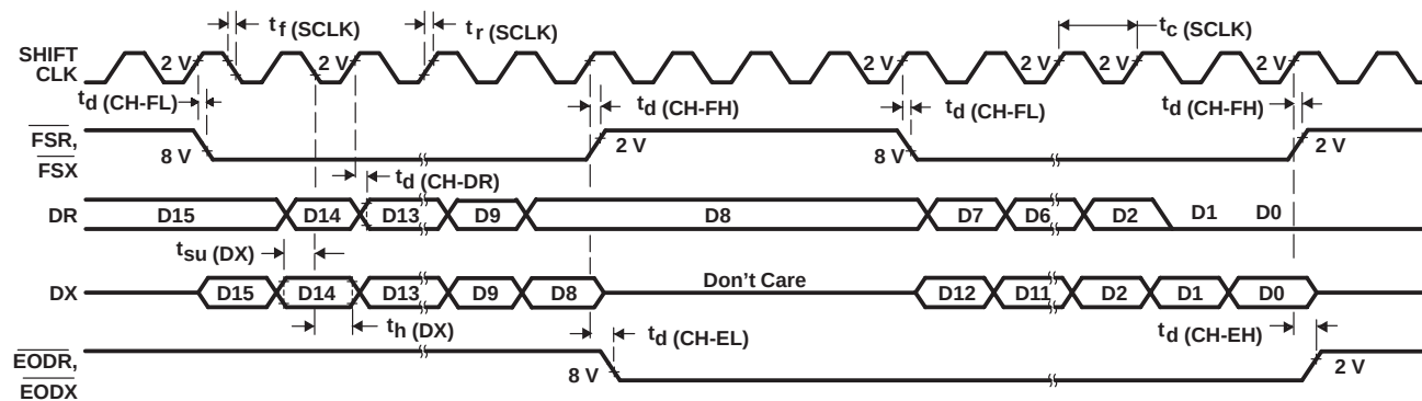
Figure 4-4. Byte-Mode Timing
