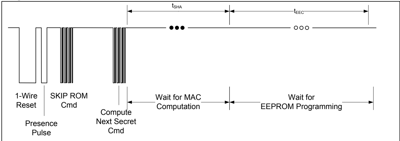
Figure 11. Compute Next Secret Function Command
