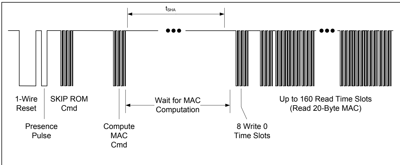
Figure 10. Compute MAC Function Command
