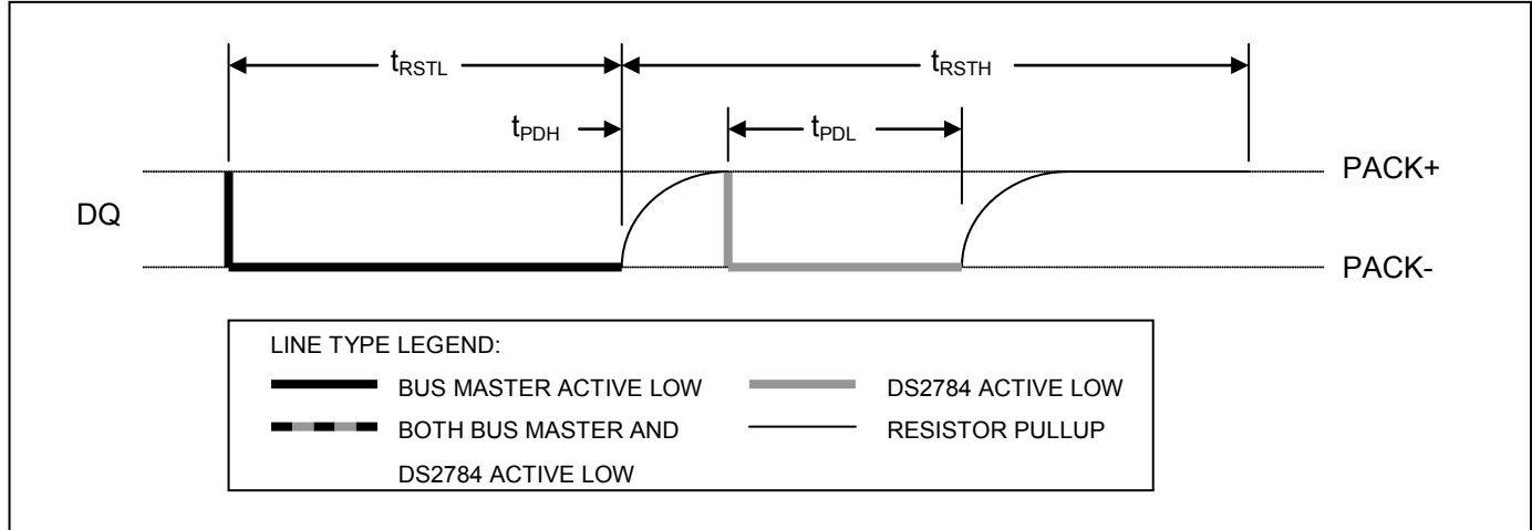
Figure 14. 1-Wire Initialization Sequence
