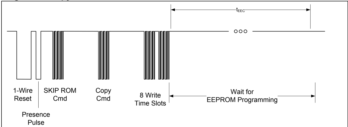
Figure 12. Copy Function Command
