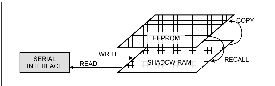
Figure 6. EEPROM Access via Shadow RAM
