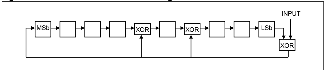
Figure 8. 1-Wire CRC Generation Block Diagram
