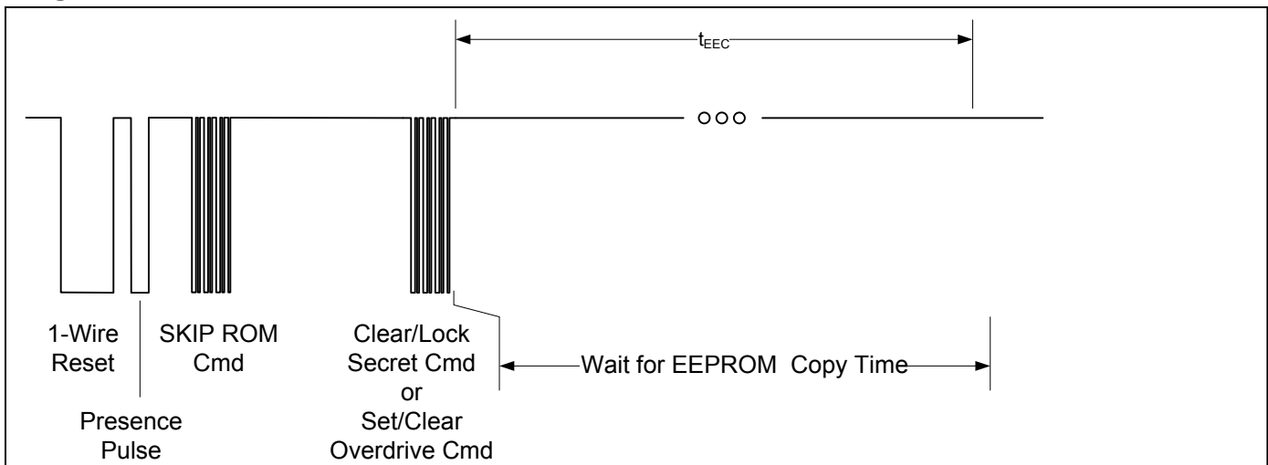
Figure 13. Clear/Lock Secret, Set/Clear Overdrive Function Commands
