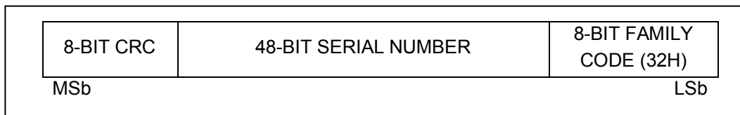
Figure 7. 1-Wire Net Address Format
