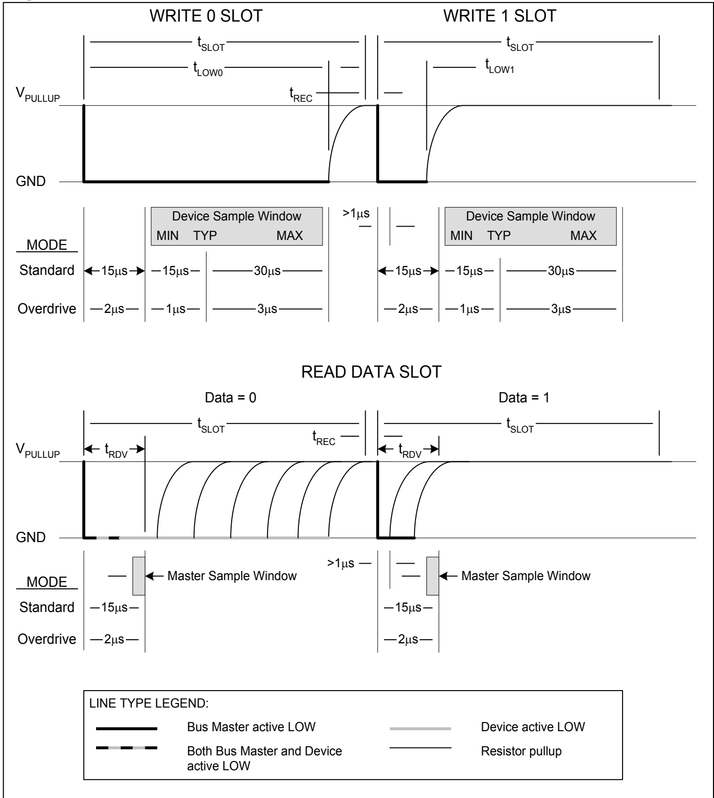
Figure 15. 1-Wire Write and Read-Time Slots
