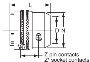
“CP” Potting Boot
