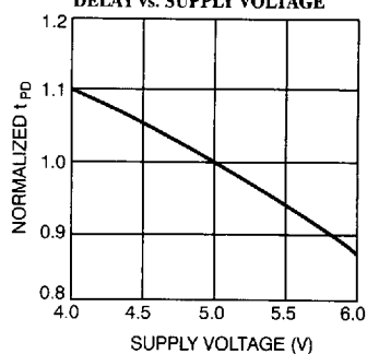
NORMALIZED PROPAGATION DELAY vs. SUPPLY VOLTAGE
