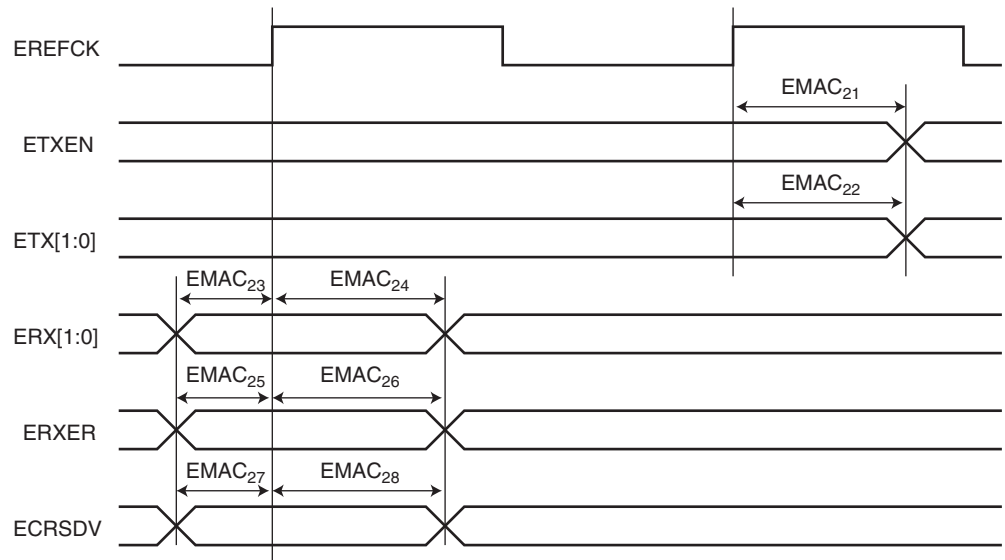
Figure 46-22. EMAC RMII Timings
