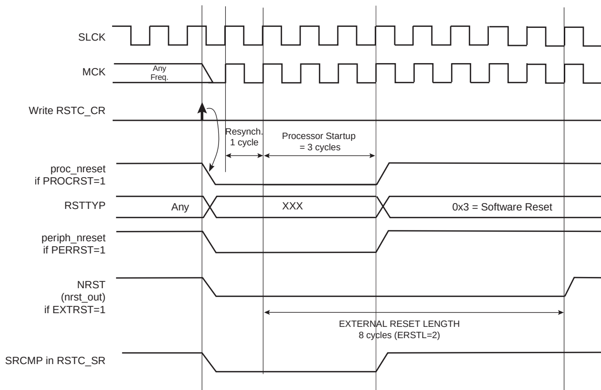
Figure 12-7. Software Reset
