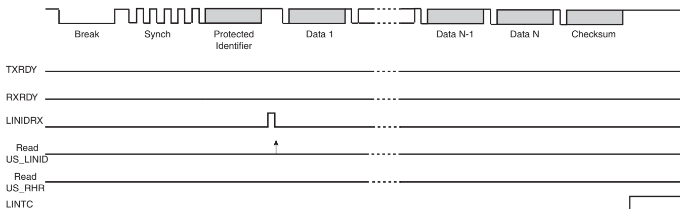
Figure 33-51. Slave Node Configuration, NACT = IGNORE
