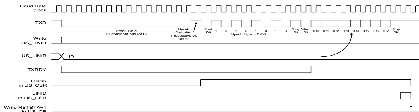
Figure 33-40. Header Transmission
