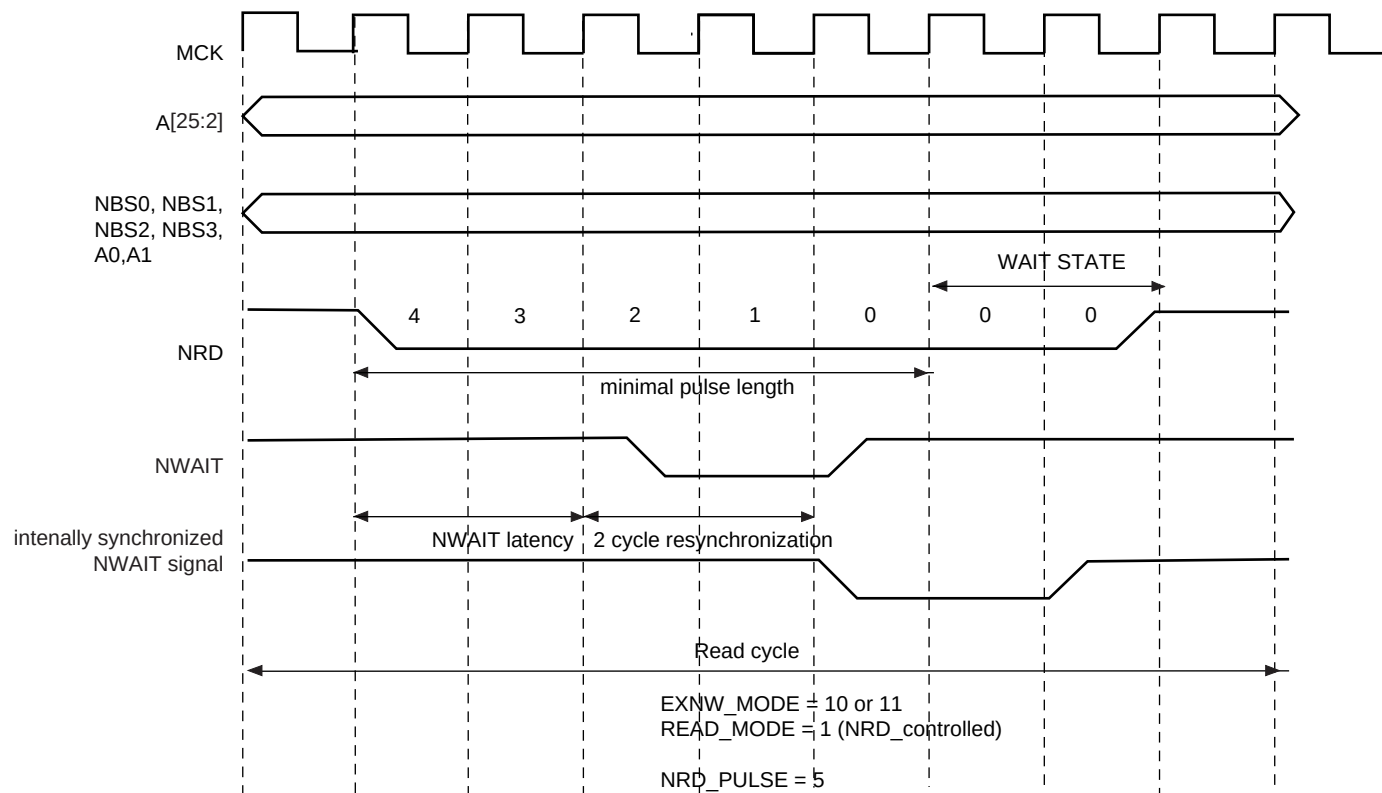
Figure 21-30. NWAIT Latency
