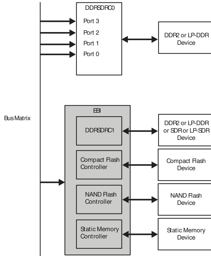
Figure 20-1. DDRSDR Controllers
