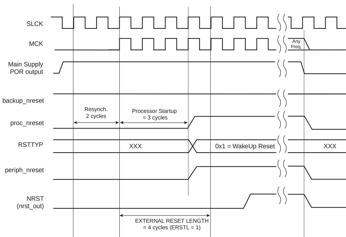
Figure 12-5. Wake-up State
