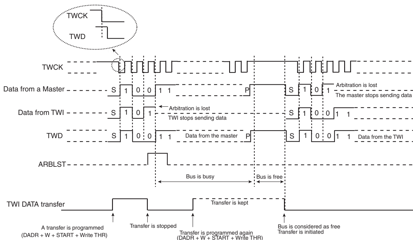
Figure 31-22. Arbitration Cases
