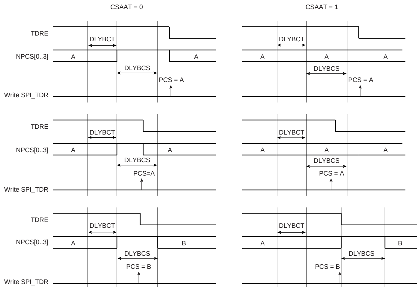
Figure 29-10. Peripheral Deselection
