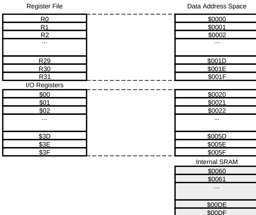
Figure 10. SRAM Organization
