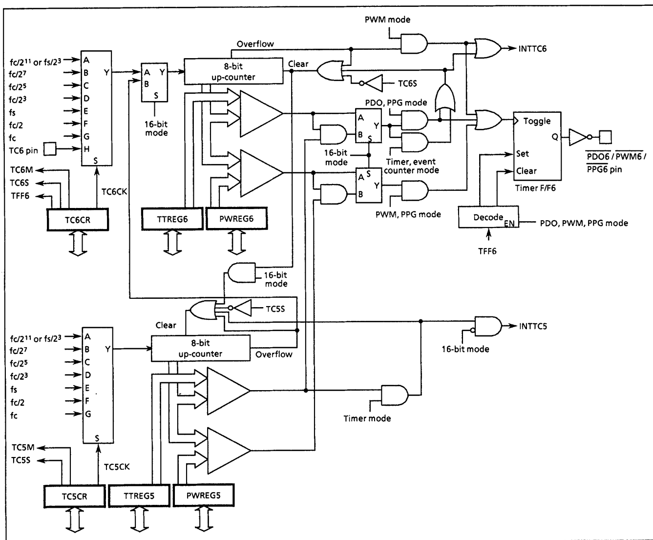
Figure 2-26. 8 bit Timer 5, 6
