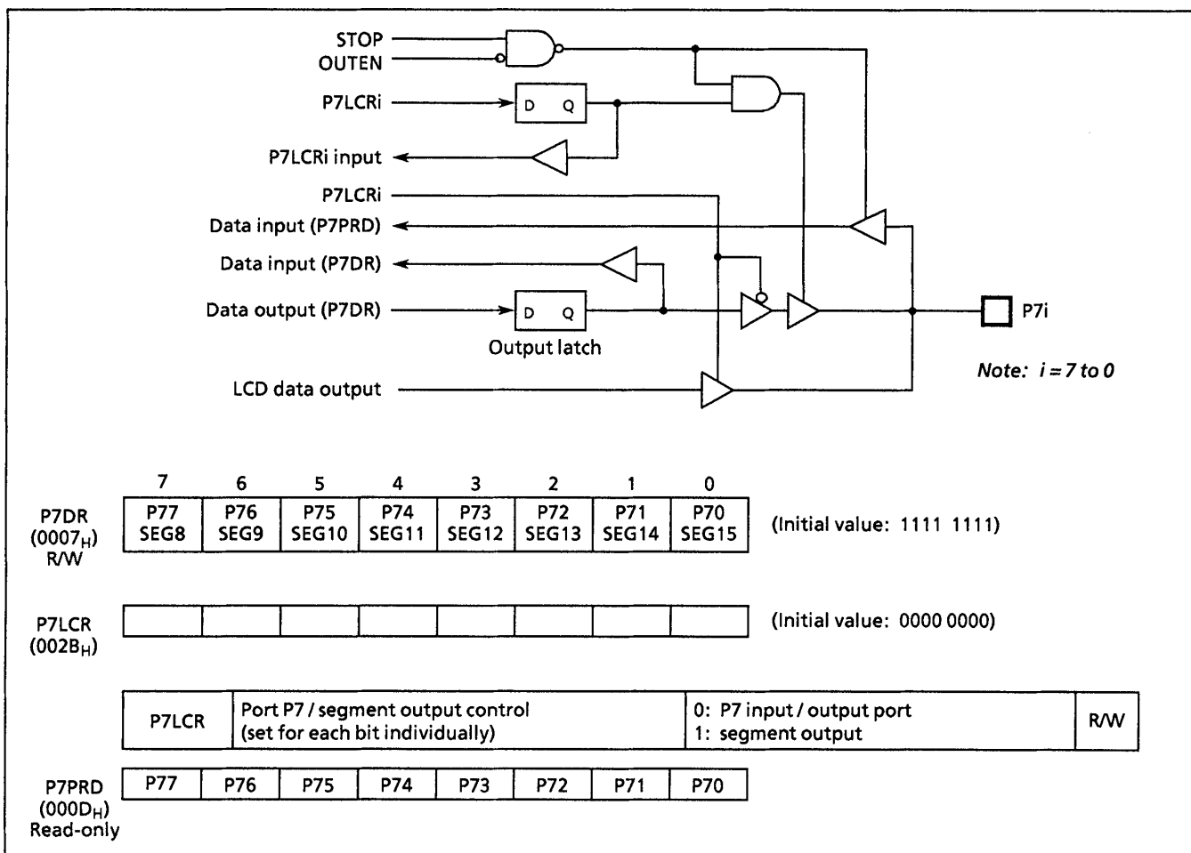
Figure 2-8. Port 7
