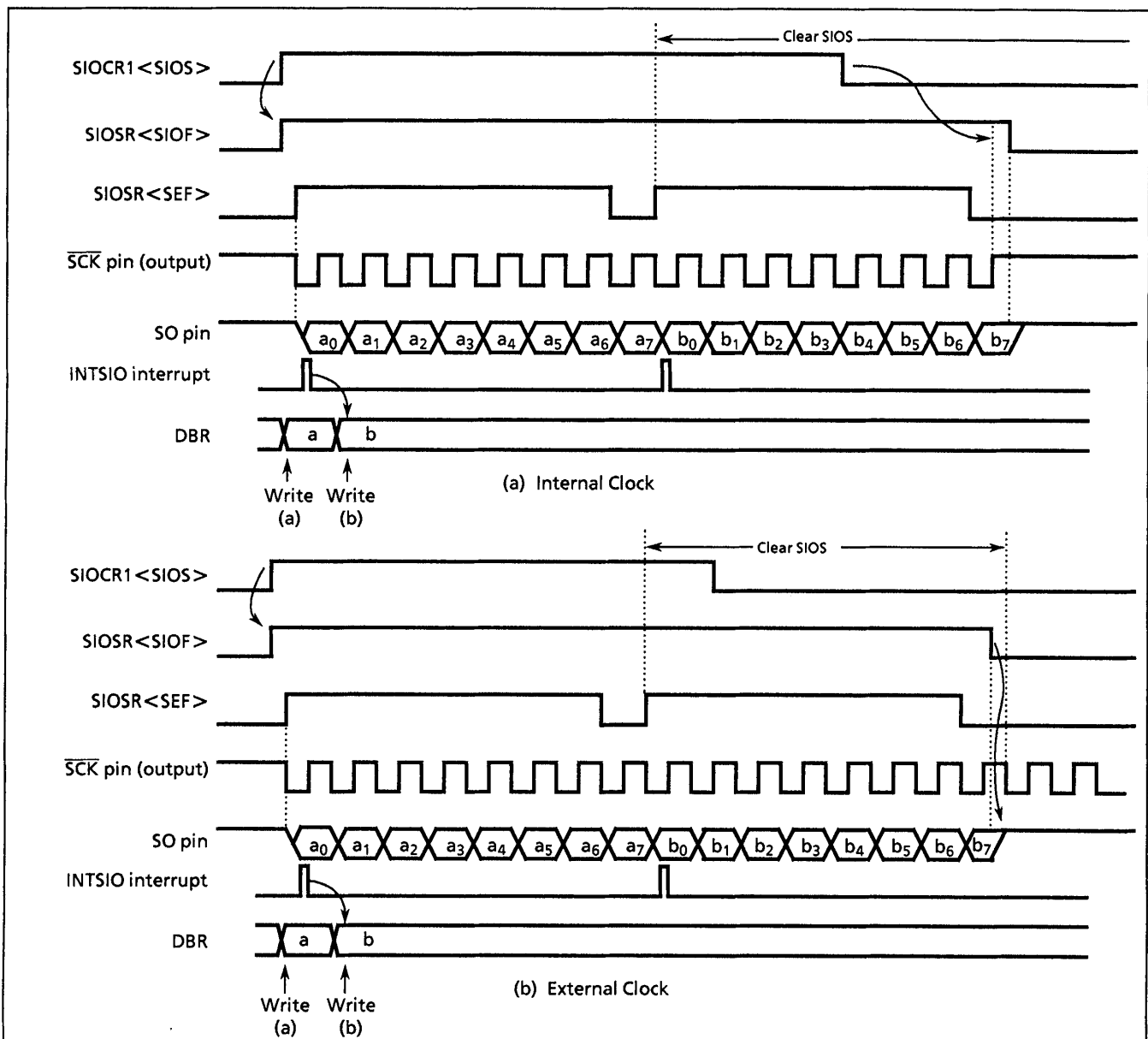
Figure 2-53. Transfer Mode (Example: 8-bit, 1 Word Transfer)
