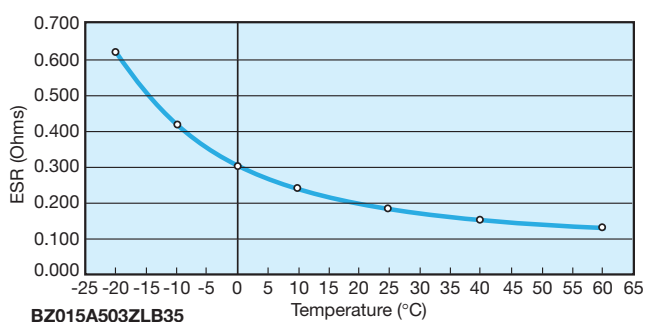
ESR Comparison
