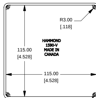
Top View Looking Inside Box
