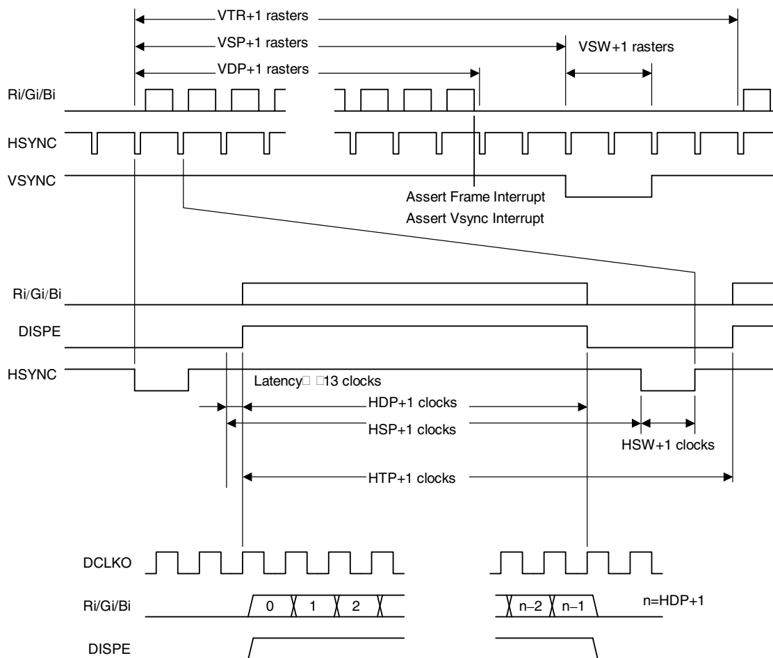
Fig. 11.10 Non-interlace Timing
