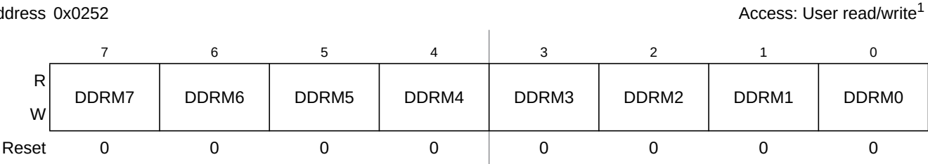
Figure 2-34. Port M Data Direction Register (DDRM)
