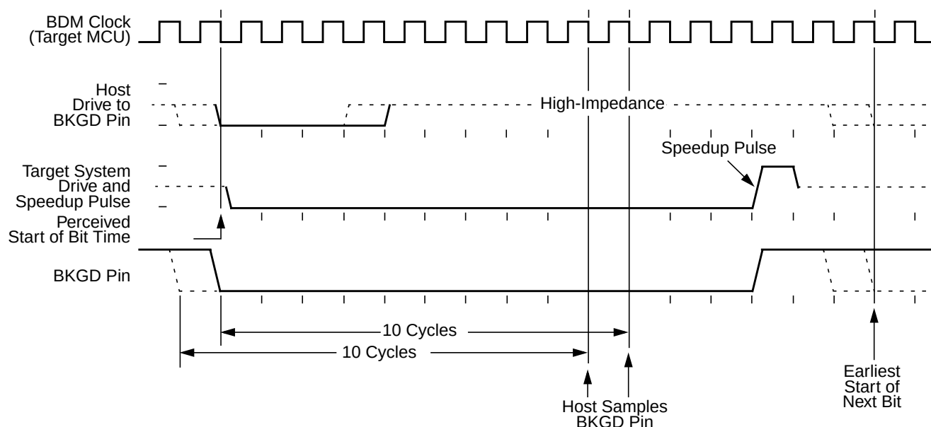
Figure 5-10. BDM Target-to-Host Serial Bit Timing (Logic 0)
