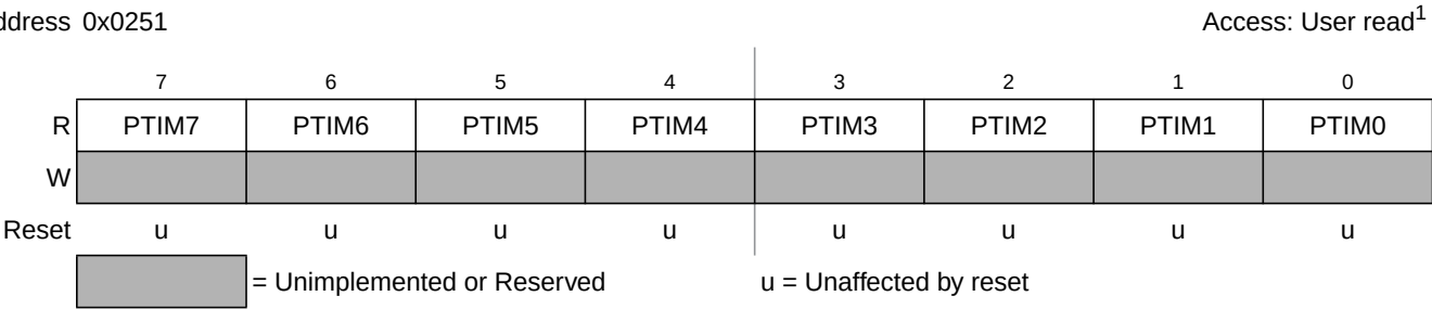
Figure 2-33. Port M Input Register (PTIM)
