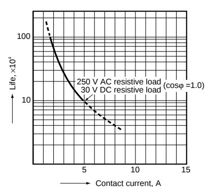
2-(1). Life curve 1 Form A Standard (5 A) type
