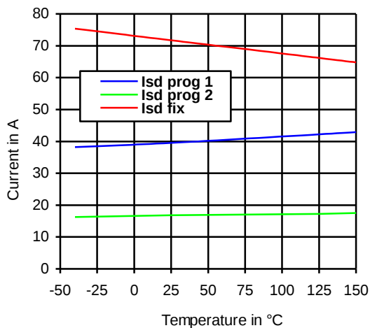
Figure 12: Current shutdown vs. temperature
