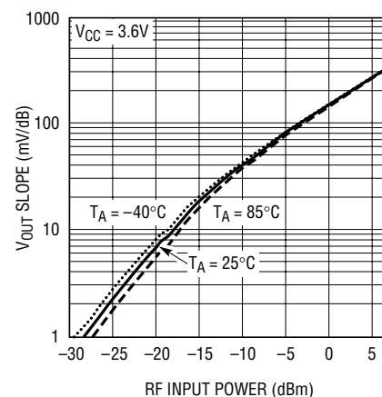
V_{\text{OUT}} Slope vs RF Input Power at 850MHz
