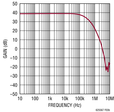
Figure 3. Gain of 100 Amplifier (3dB Bandwidth of 200kHz on 130 \mu A Supply Current)
