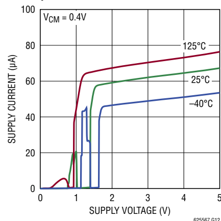
Supply Current vs Supply Voltage per Channel
