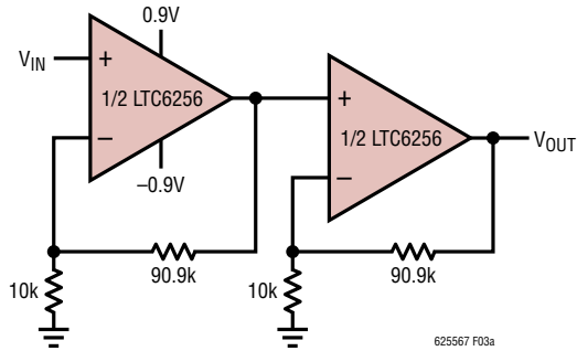
200kHz 130 \mu A Gain-of-100 Amplifier
