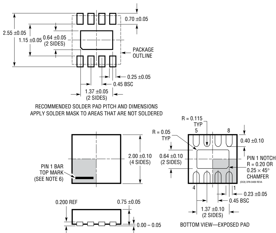
DC8 Package 8-Lead Plastic DFN (2mm × 2mm) (Reference LTC DWG # 05-08-1719 Rev A)
