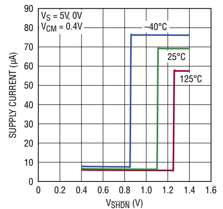
Supply Current vs \overline{\text{SHDN}} Pin Voltage
