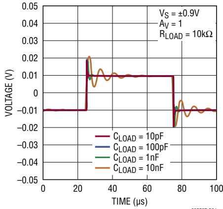
Small-Signal Response
