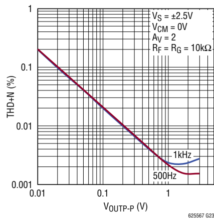
Total Harmonic Distortion and Noise
