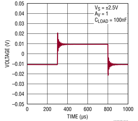
Small-Signal Response
