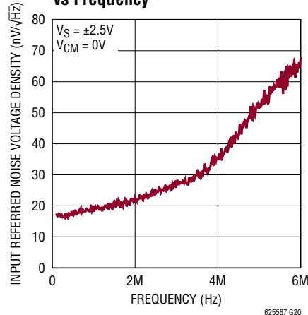
Wide Band Noise Voltage Density vs Frequency
