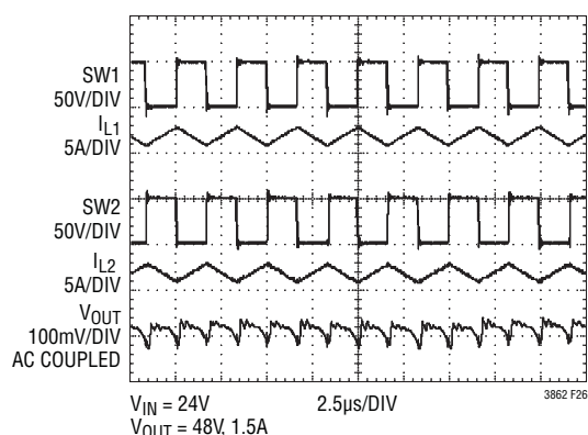
Figure 26. LTC3862 Switching Waveforms for Boost Converter
