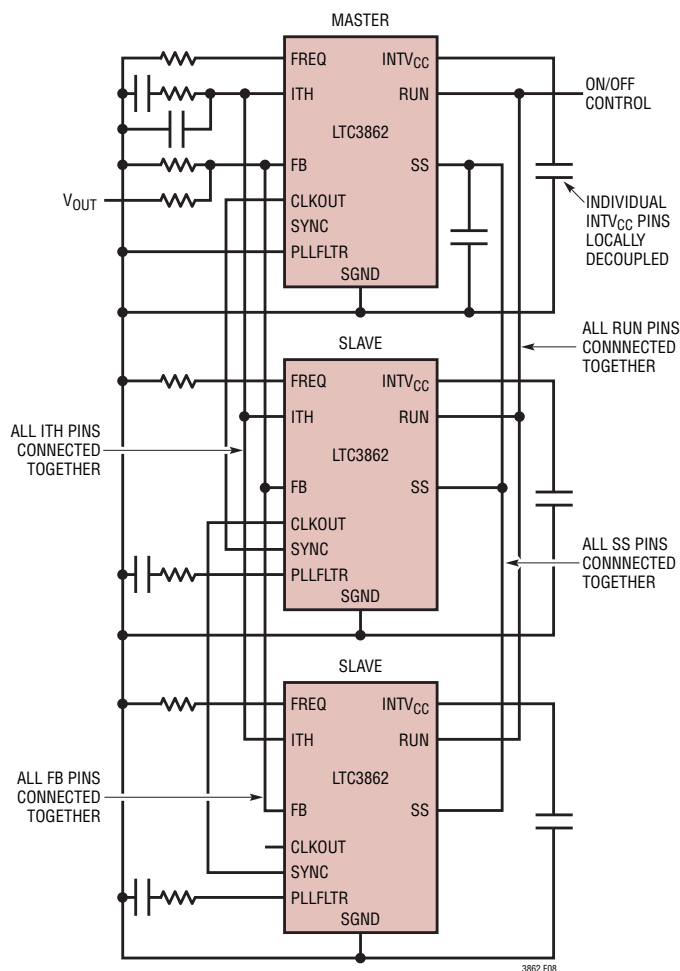
Figure 8. LTC3862 Error Amplifier Configuration for Multi-Phase Operation
