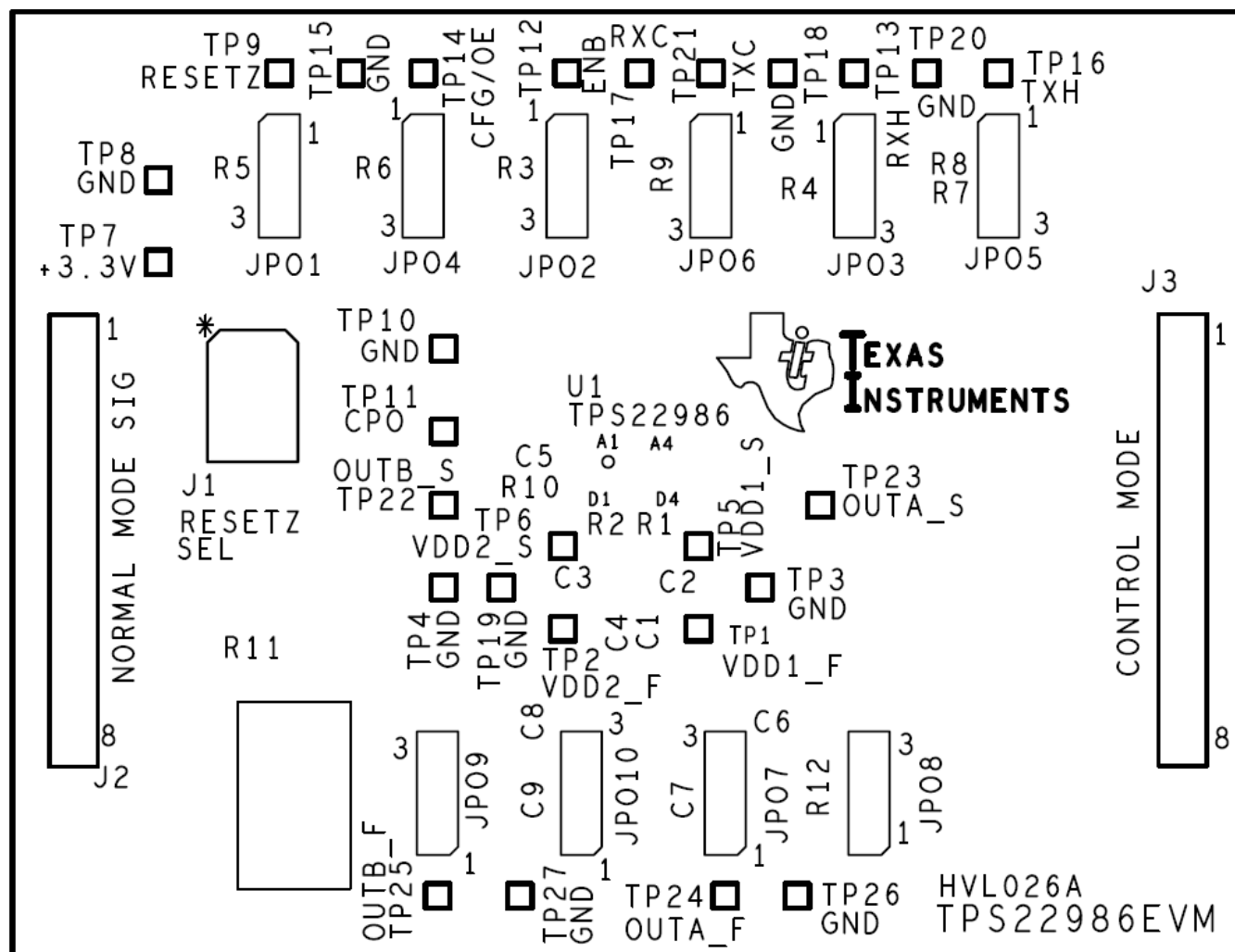
Figure 1. Top Layer Assembly
