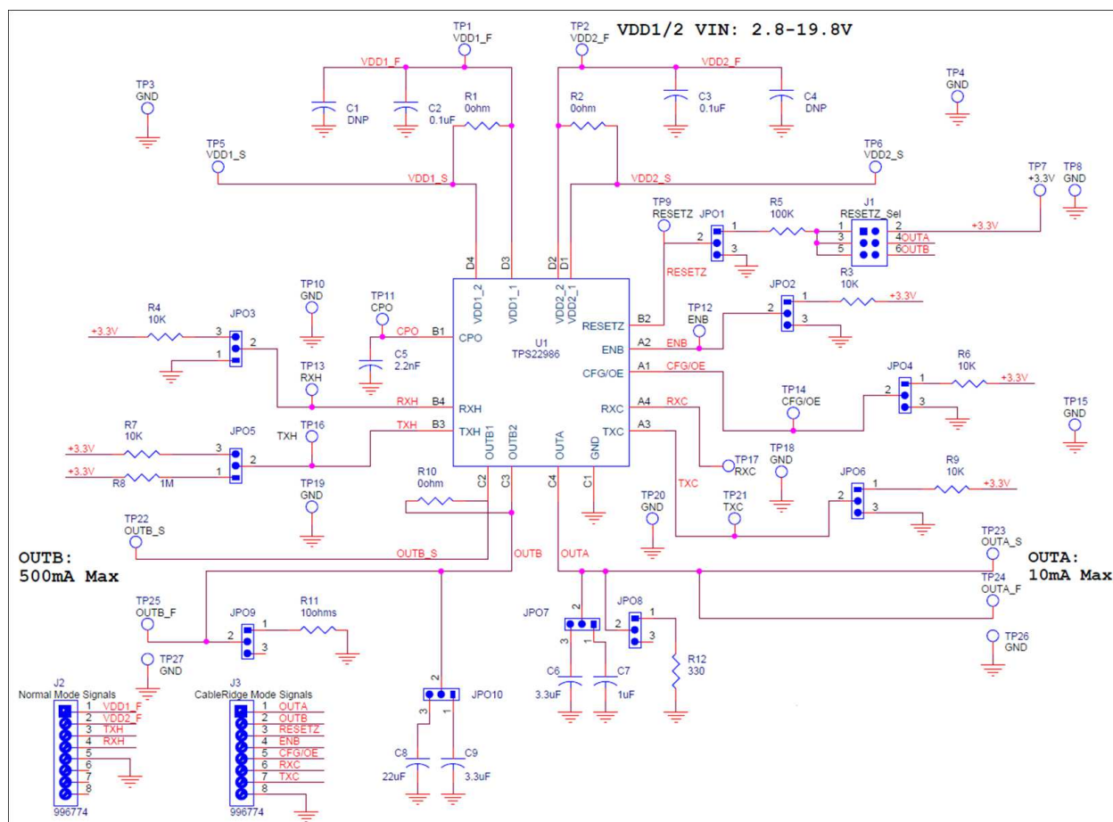
Figure 4. TPS22986EVM Schematic
