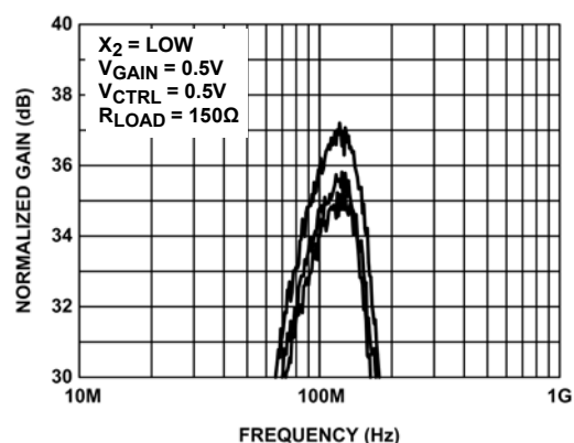
FIGURE 6. CHANNEL MISMATCH
