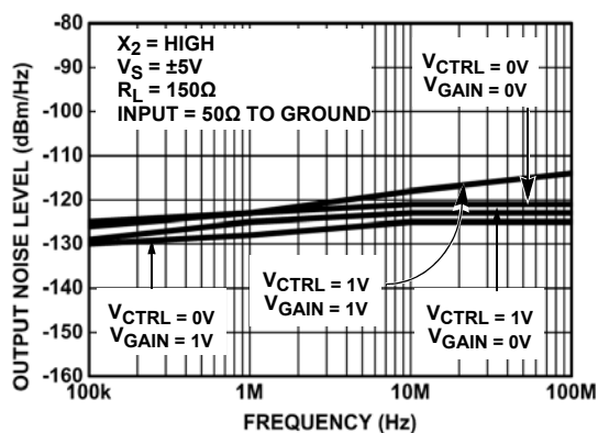
FIGURE 10. OUTPUT NOISE
