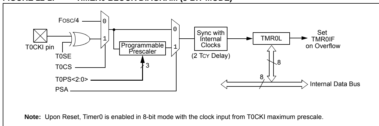
FIGURE 12-1: TIMER0 BLOCK DIAGRAM (8-BIT MODE)
