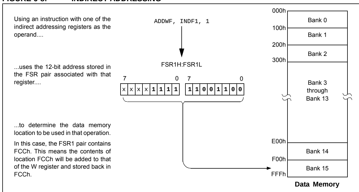
FIGURE 6-8: INDIRECT ADDRESSING
