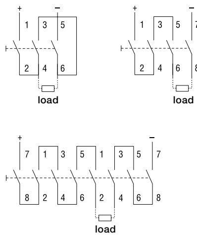
Circuit diagrams
