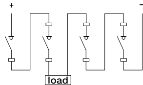
Circuit diagrams
