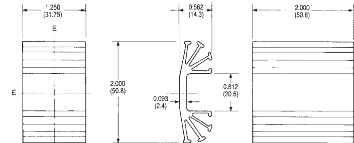
603 SERIES (EXTRUSION PROFILE 1284)
