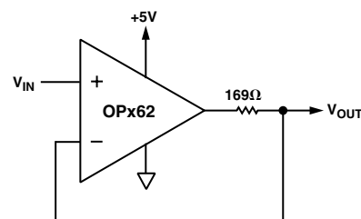
Figure 29. Output Short-Circuit Protection
