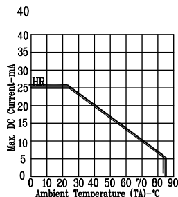
Fig5. MAX. ALLOWABLE DC CURRENT VS. AMBIENT TEMPERATURE.
