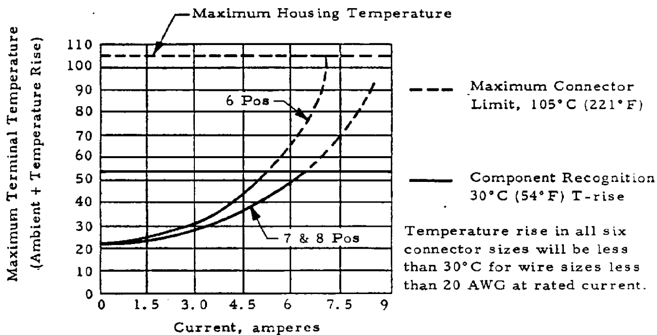
6, 7 and 8 Position Connectors With 20 AWG Wire
