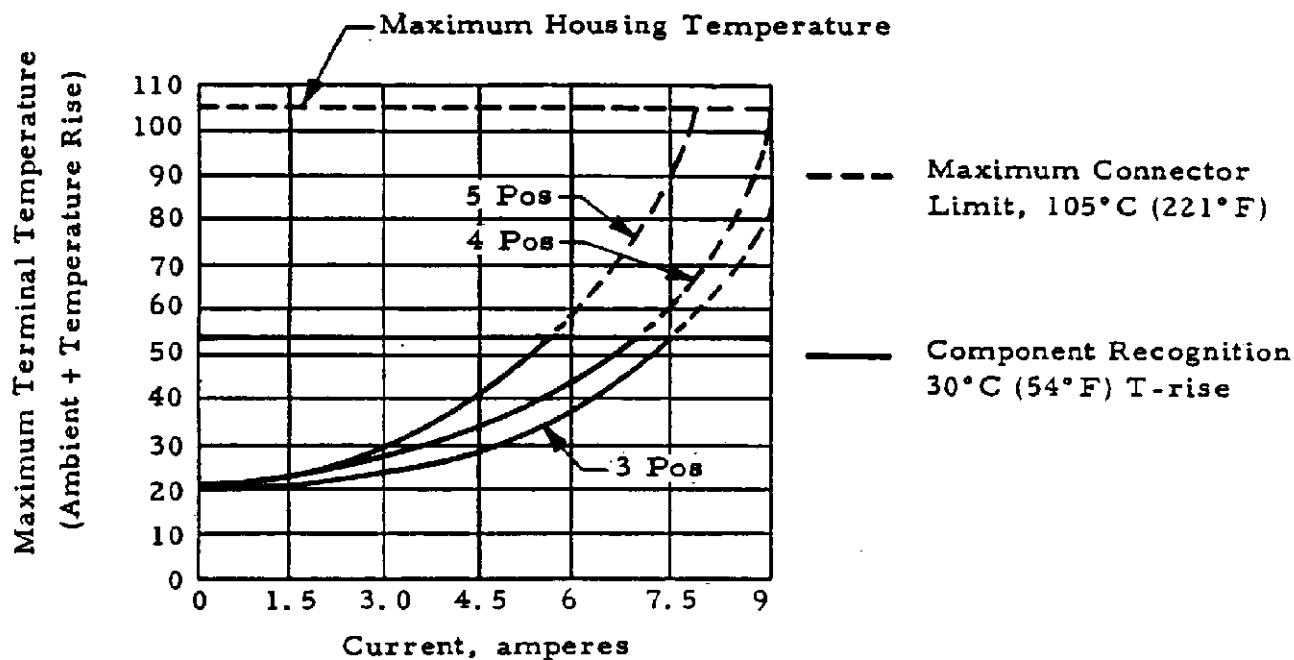
3, 4 and 5 Position Connectors With 20 AWG Wire
