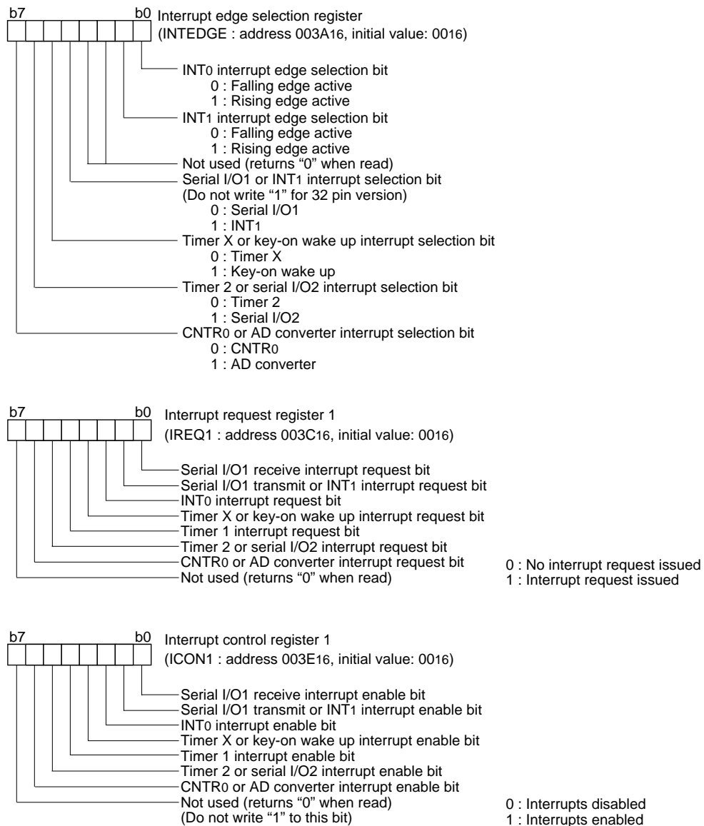
Fig. 18 Structure of Interrupt-related registers
