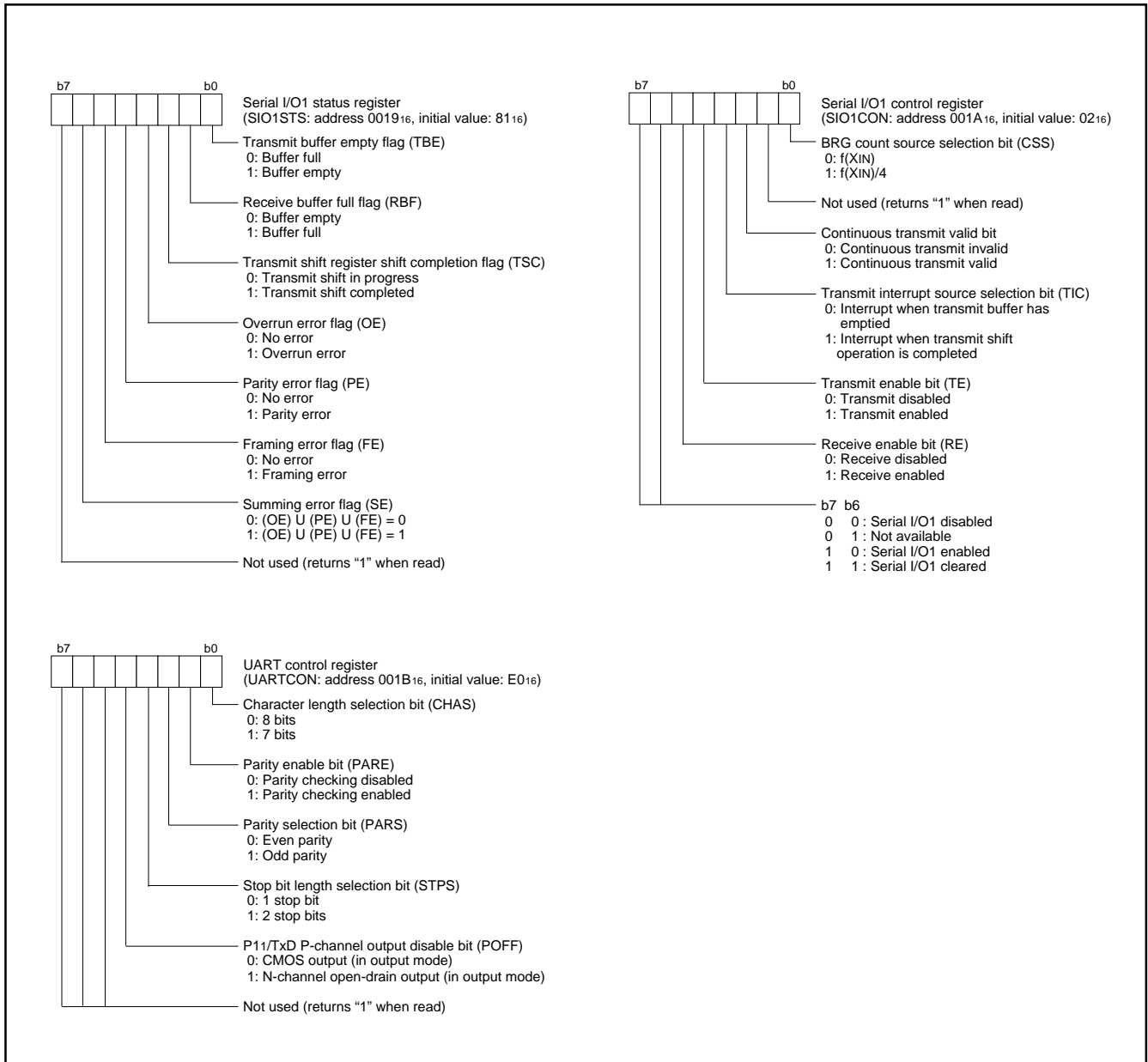
Fig. 26 Structure of serial I/O-related registers (1)
