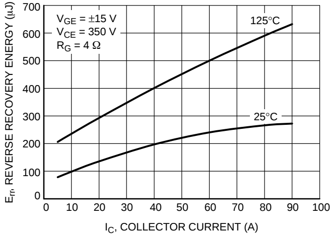
Figure 29. Typical Reverse Recovery Energy vs. I_C
