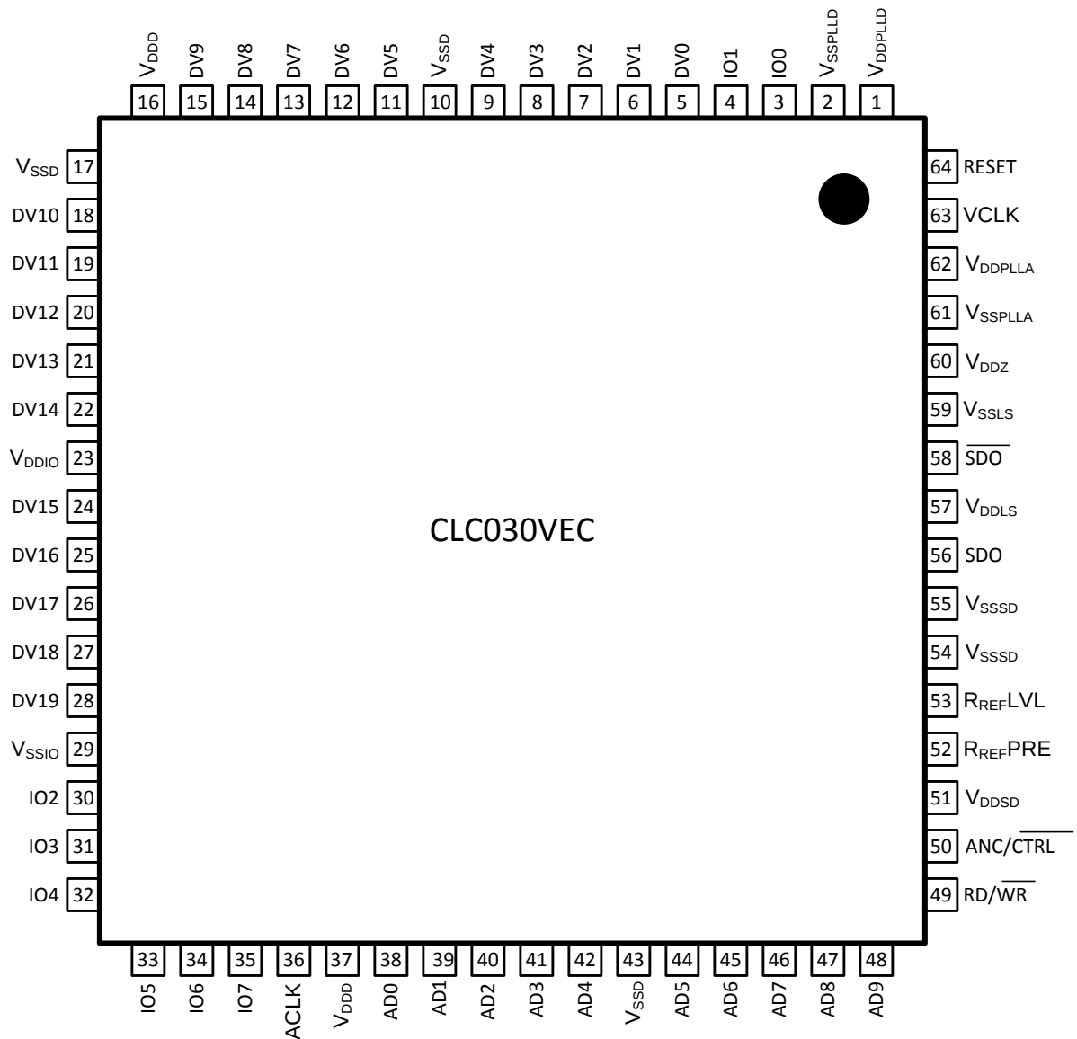
Figure 1. 64-Pin TQFP
