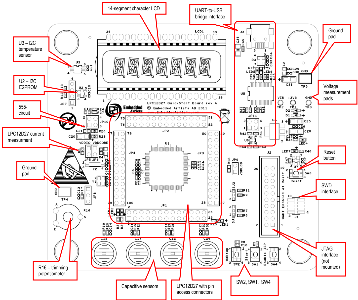
Figure 2 – LPC12D27 QuickStart Board Overview
