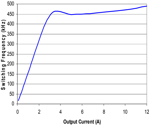
Figure 2. Switching Frequency Vs Output Current
