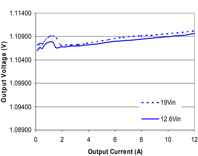
Figure 5. Output Voltage Regulation Vs Output Current
