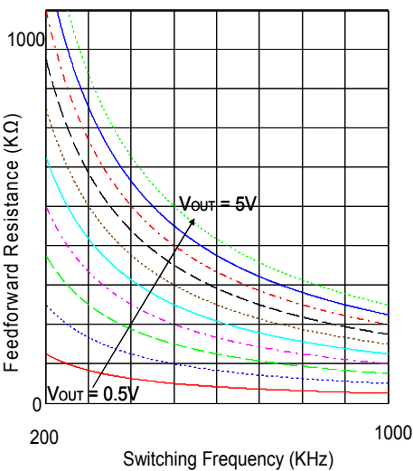
Figure 1. Feedforward Resistance Vs Switching Frequency: 0.5V VOUT step
