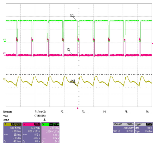
CH1: Vout (50mV/div); CH2: Phase (10V/div) CH4: CPO (2V/div); Time: 2uS/div Figure 13: Charge Pump On at I OUT = 3A
