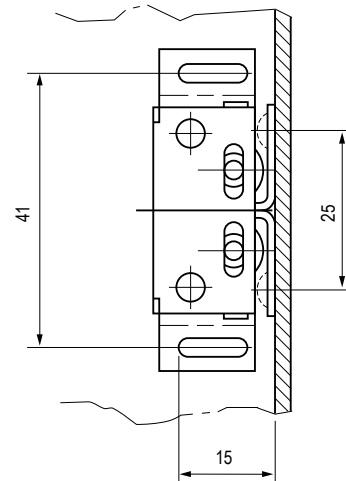
取付図 Installation Layout
