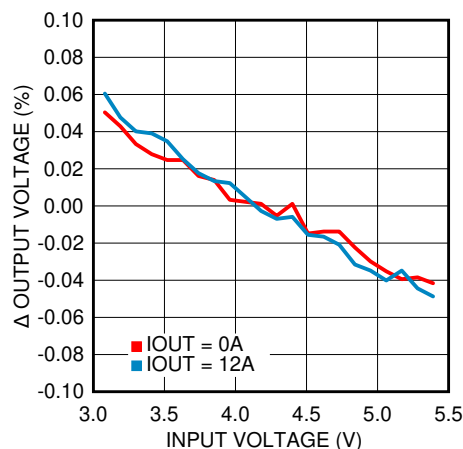
Figure 8-11. Line Regulation
