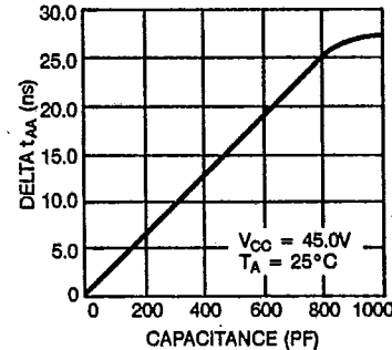
TYPICAL ACCESS TIME CRANGE vs. OUTPUT LOADING
