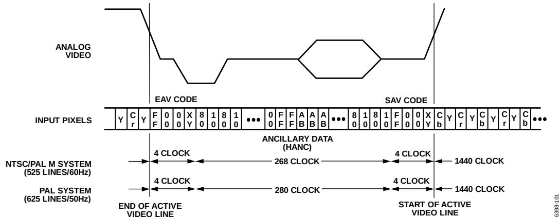
Figure 99. SD Slave Mode 0
