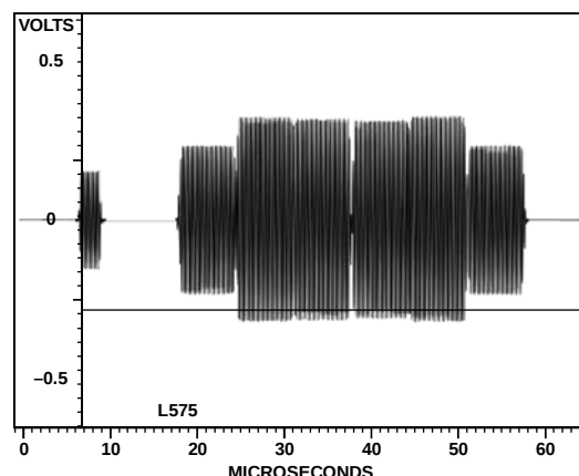
Figure 131. PAL Luma
