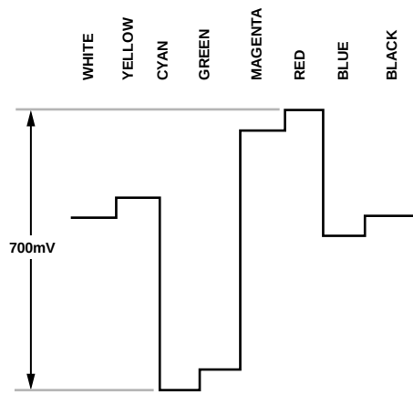
Figure 117. Pr Levels—PAL
