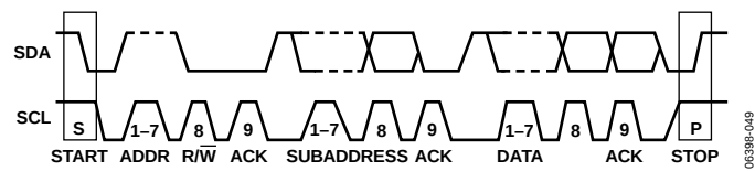
Figure 49. I 2 C Data Transfer
