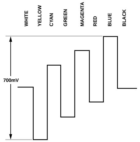
Figure 118. Pb Levels—PAL
