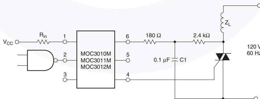
Figure 11. Inductive Load with Sensitive Gate Triac (I GT ≤ 15 mA)
