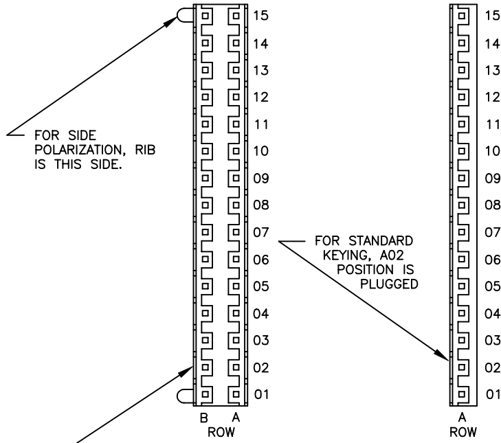
CONTACT NUMBERING SYSTEM AS VIEWED FROM CONTACT INSERTION END.
