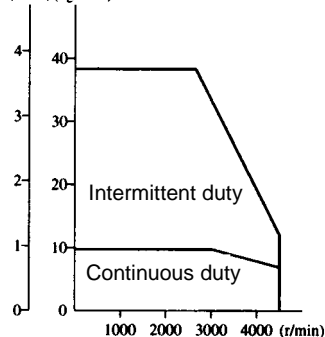
R88M-U30030LA (N·m)(kgf·cm)
