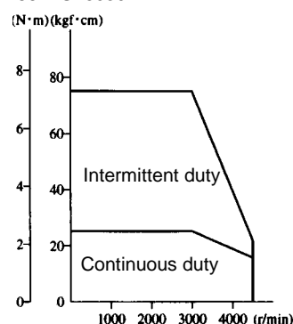
R88M-U75030HA (N·m)(kgf·cm)
