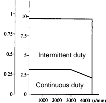
R88M-U10030LA (N·m)(kgf·cm)
