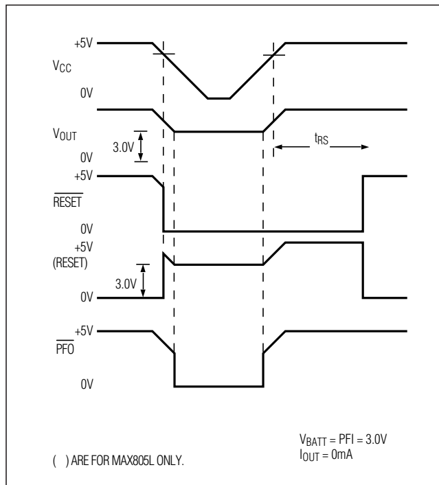
Figure 2. Timing Diagram
