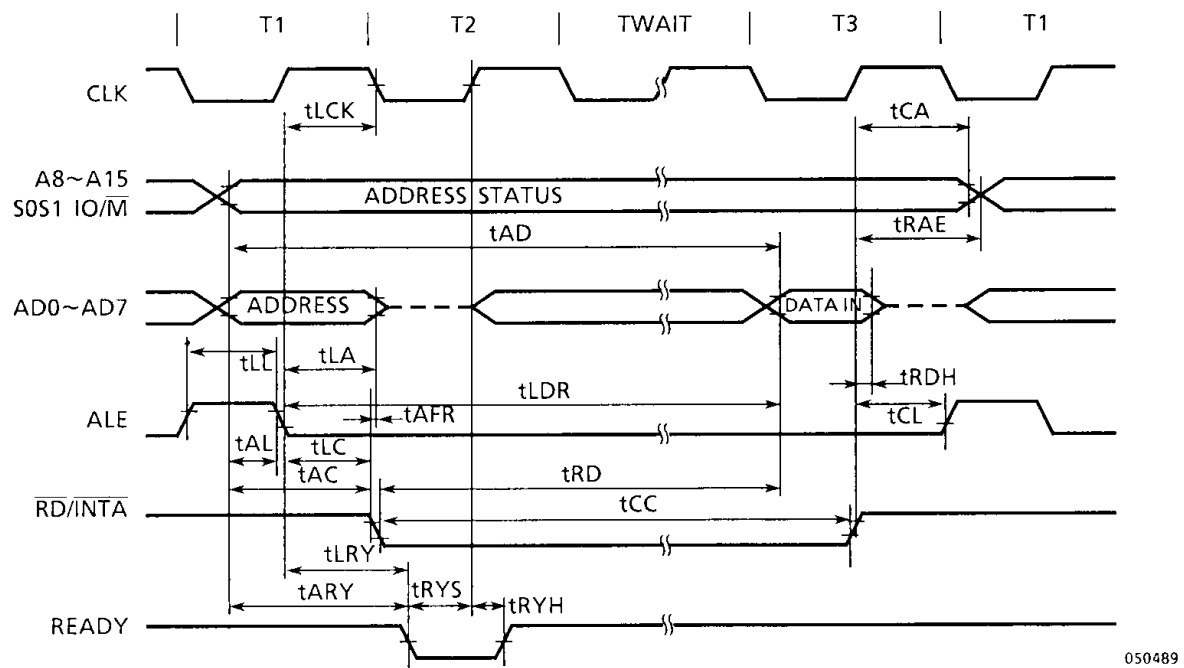
Figure 12.4 Read Operation with Wait Cycle (Typical) - Same Ready Timing Applied to Write Operation
