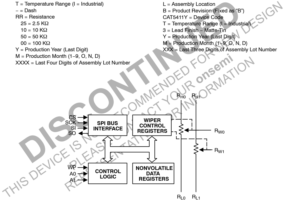
Figure 1. Functional Diagram
