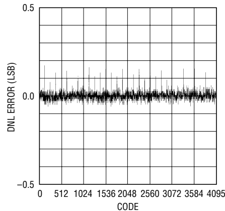
LTC1451 Differential Nonlinearity (DNL)
