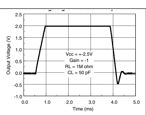
Figure 16. Large signal transient response
