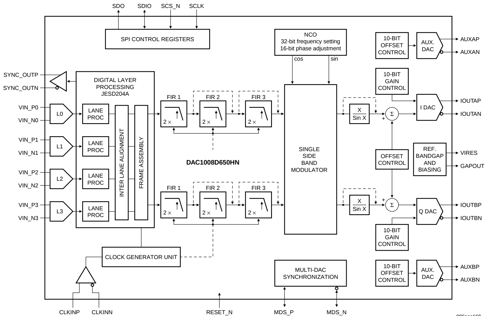
Fig 1. Block diagram
