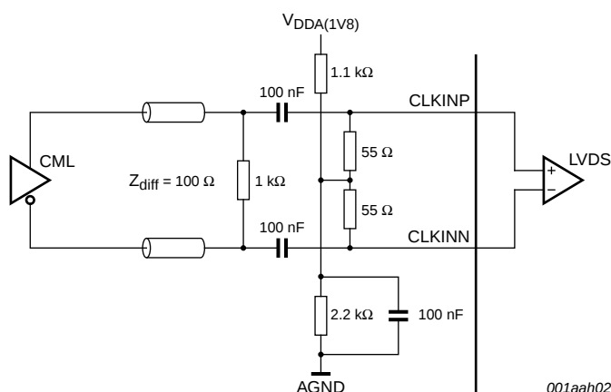
Fig 16. Interfacing CML to LVDS
