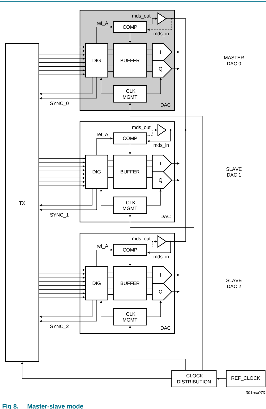
Fig 8. Master-slave mode
