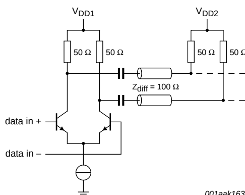
Fig 6. AC coupling
