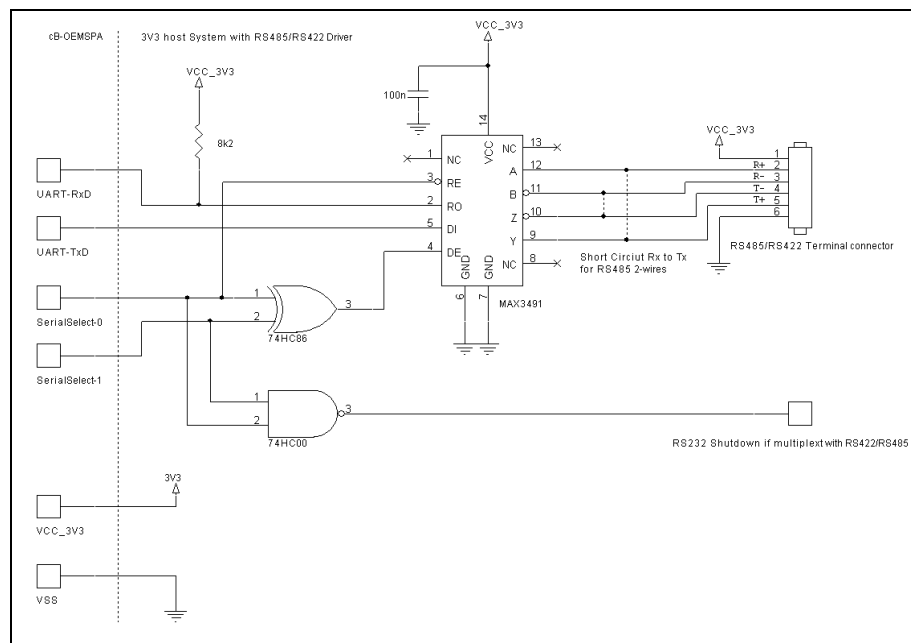
Figure 17: A complete RS422/RS488 transceiver design.
