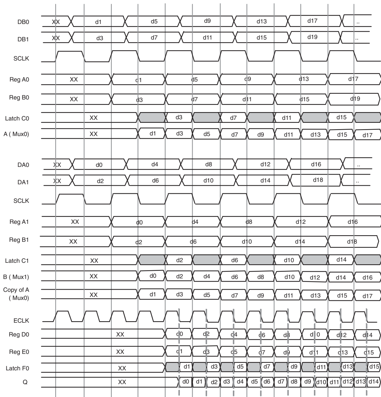
Figure 12-40. ODDRX2B Waveform
