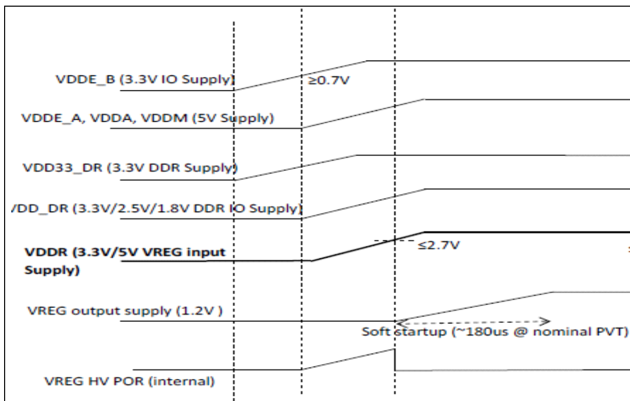
Figure 6. Power-up sequencing
