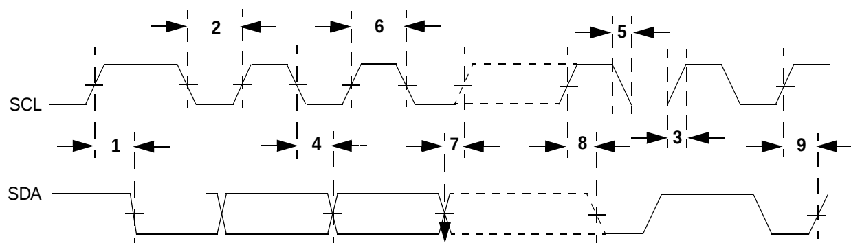
Figure 41. I²C input/output timing
