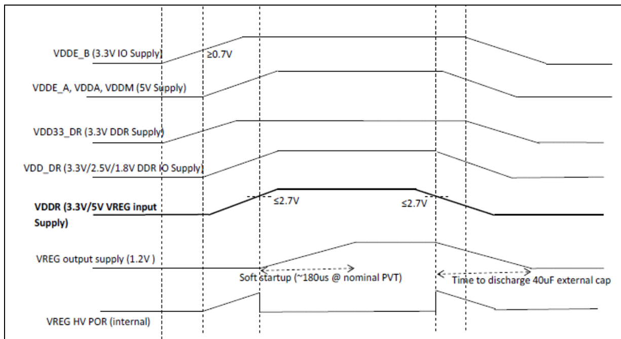
Figure 7. Power-down sequencing
