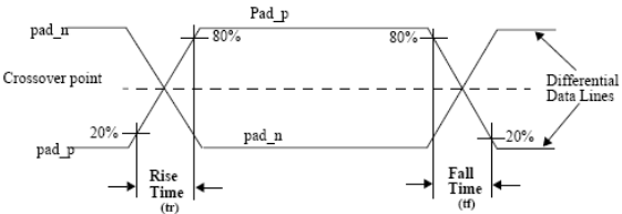
Figure 45. Rise/fall transition, part 1
