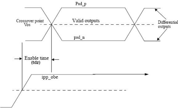
Figure 46. Rise/fall transition, part 2
