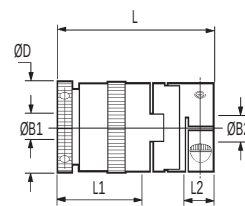
Ref. 267 (2 plate) 269 (6 plate) Basic clutch + Oldham (clamp) coupling
