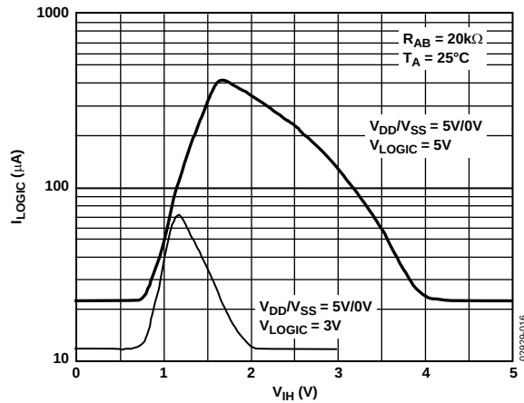
Figure 16. V_{\text{LOGIC}} Supply Current vs. Digital Input Voltage
