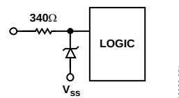
Figure 51. ESD Protection of Digital Pins
