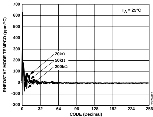
Figure 17. Rheostat Mode Tempco \Delta R_{\text{WB}}/\Delta T vs. Code, V_{\text{DD}}/V_{\text{SS}} = \pm 5V
