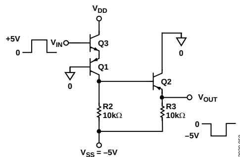
Figure 50. Level Shift for Bipolar Potential Operation
