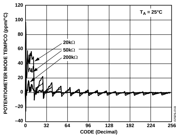
Figure 18. Potentiometer Mode Tempco \Delta V_{\text{WB}}/\Delta T vs. Code, V_{\text{DD}}/V_{\text{SS}} = \pm 5V
