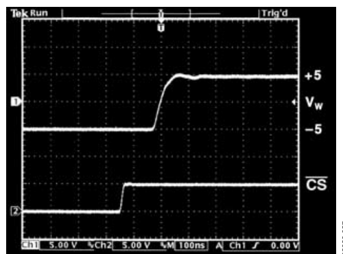
Figure 27. Large Signal Settling Time
