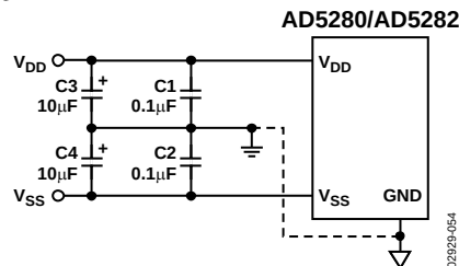
Figure 53. Power Supply Bypassing
