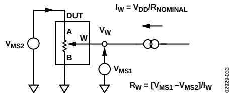
Figure 33. Wiper Resistance
