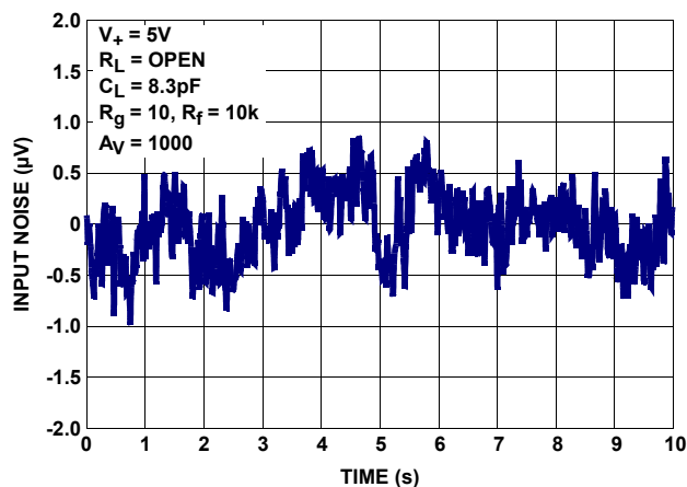
FIGURE 17. INPUT VOLTAGE NOISE 0.1Hz TO 10Hz
